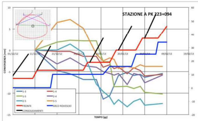
Radial displacements
