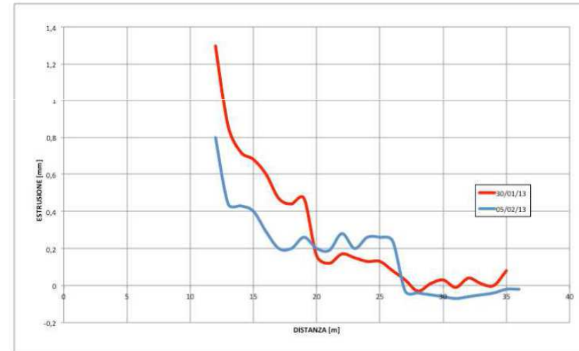
Excavation face
